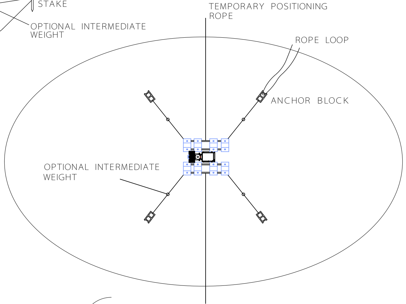
FIGURE 3, TOP VIEW
